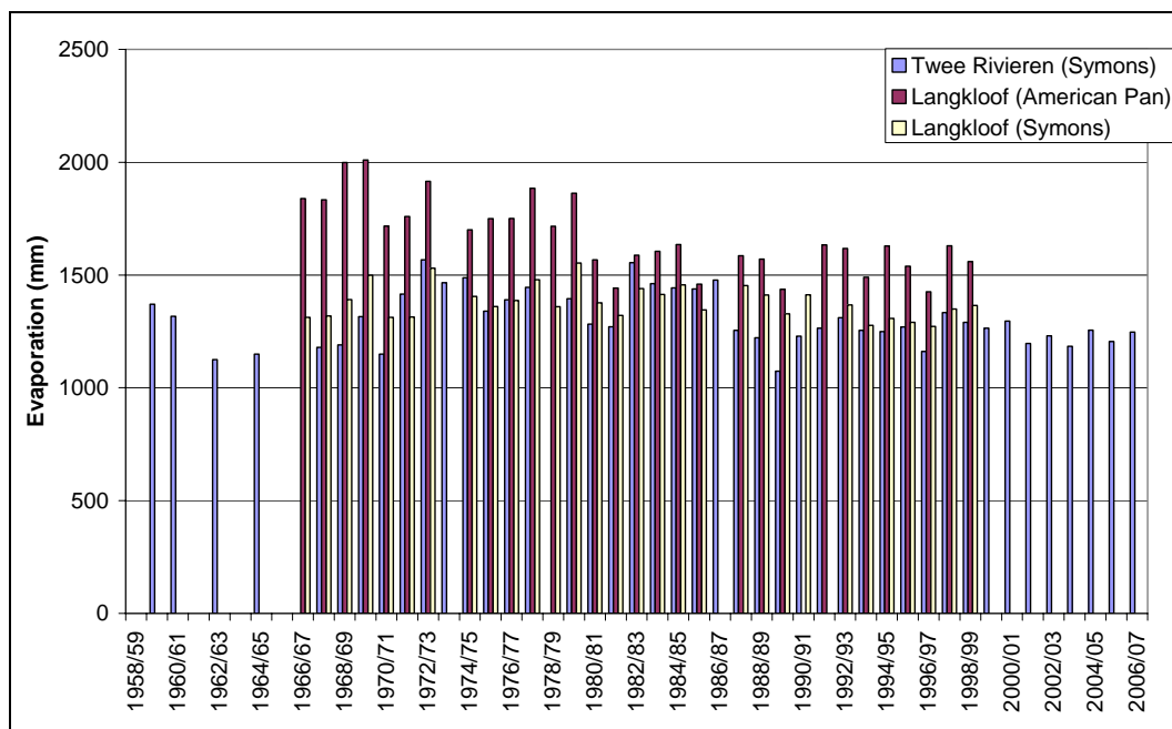
Figure 4. Annual and spatial variability of the potential evapotranspiration.
