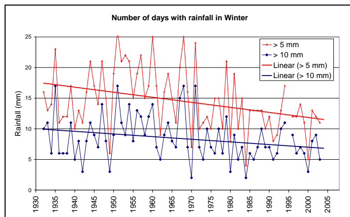
Rainfall trend Zuurans (Kouga River catchment)
