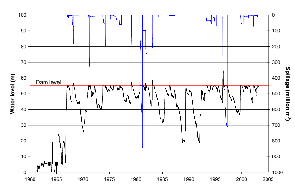
Figure 18. Water levels and spillage of the Kouga Dam
